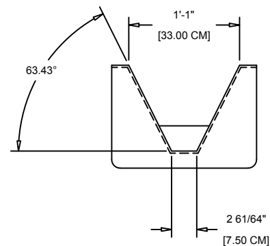
END ELEVATION VIEW
