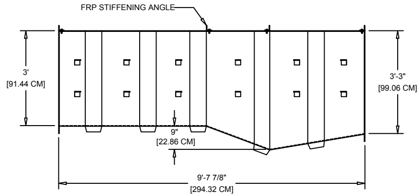
ELEVATION VIEW
