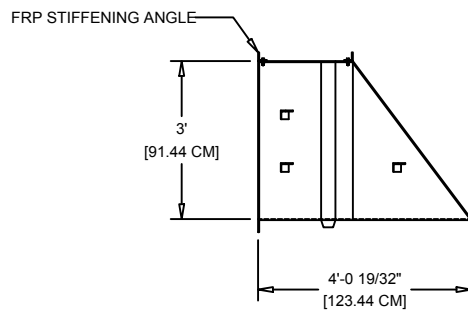
ELEVATION VIEW
