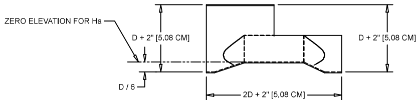
ELEVATION VIEW
