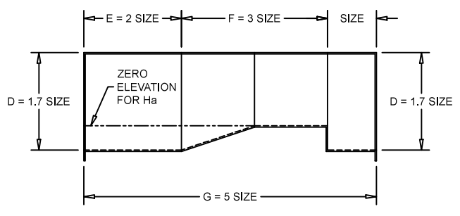
ELEVATION VIEW
