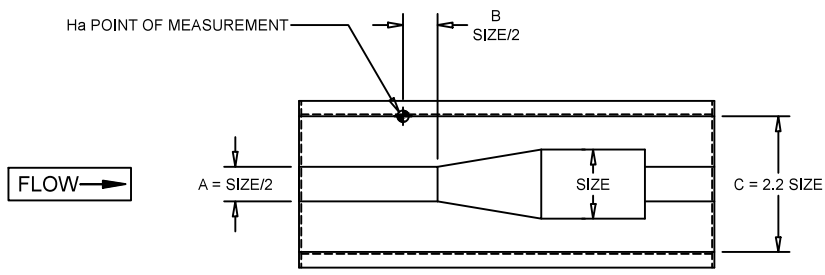
PLAN VIEW
