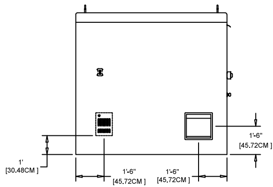
LEFT ELEVATION VIEW
