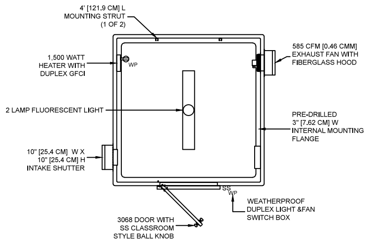
PLAN VIEW
