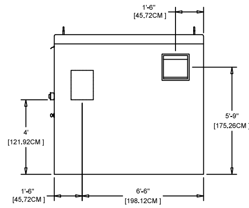
RIGHT ELEVATION VIEW
