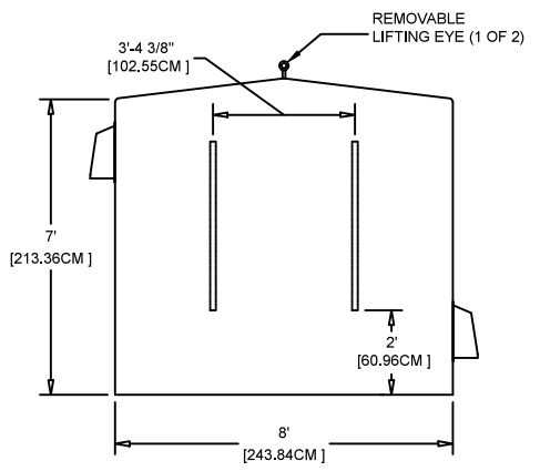
REAR ELEVATION VIEW
